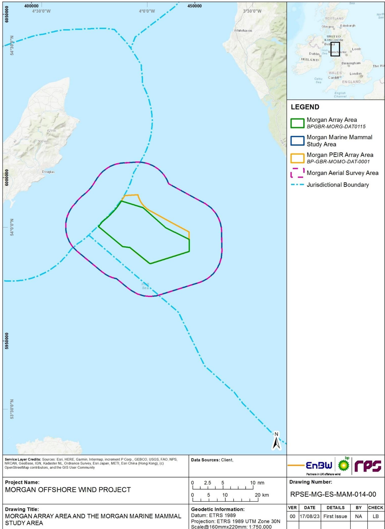
Figure 1.1: Morgan Array Area and Morgan marine mammal study area.
