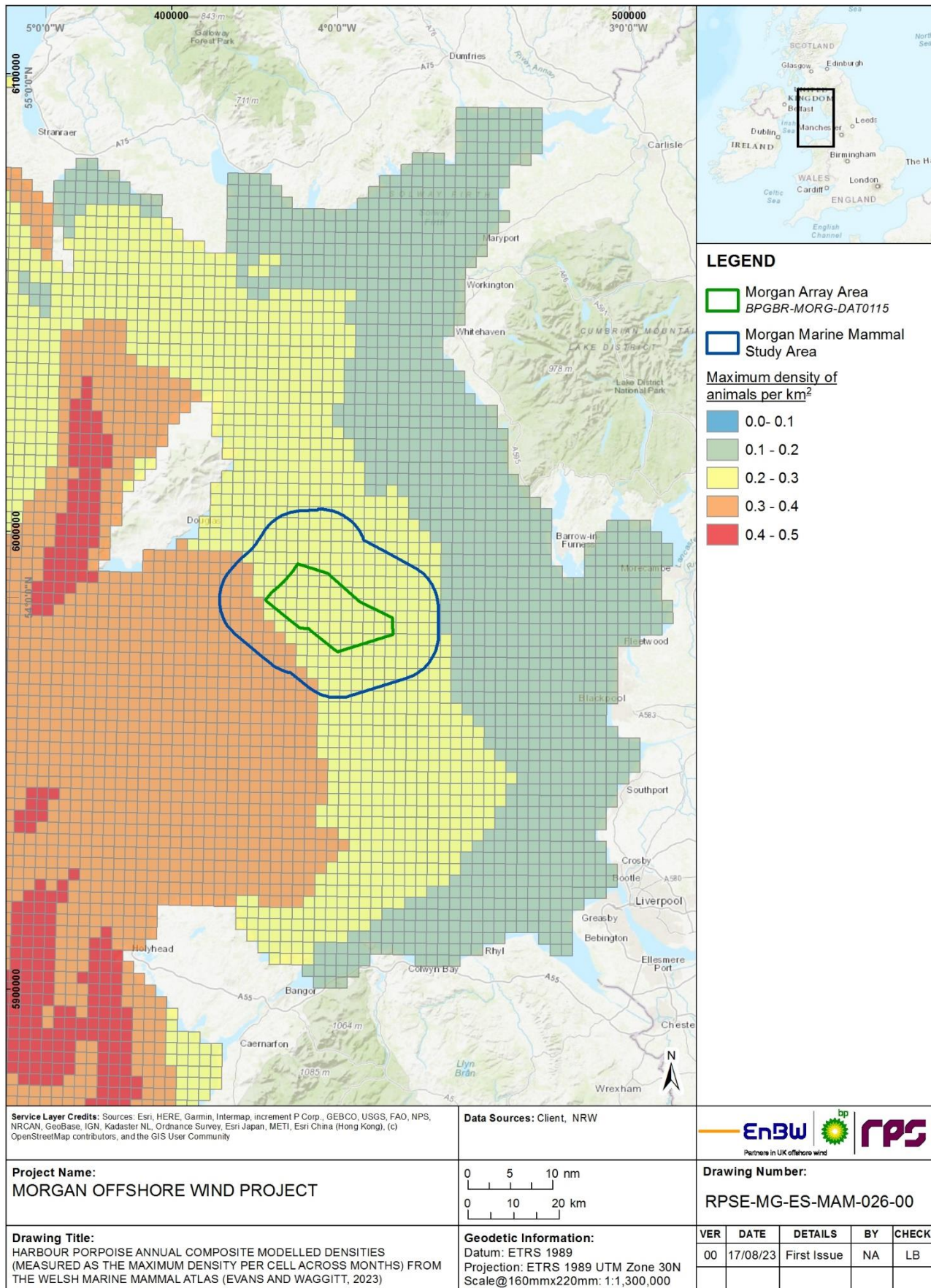
Figure 1.28: Harbour Porpoise annual composite modelled densities (measured as the maximum density per cell across months) from the Welsh Marine Mammal Atlas (Evans and Waggitt, 2023).
