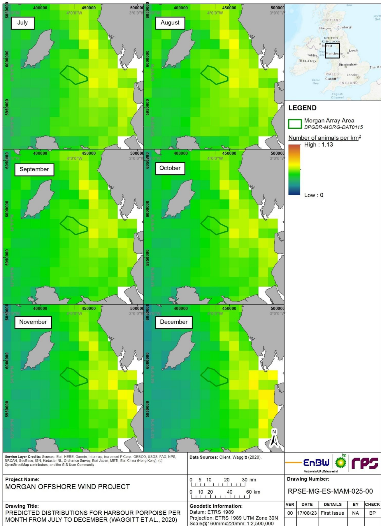
Figure 1.27: Predicted distributions for harbour porpoise per month from July to December (Waggit et al., 2020).
